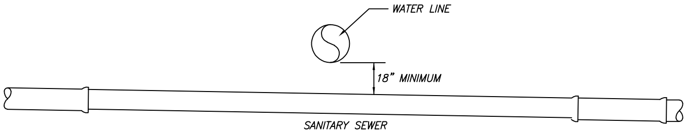
SECTION VIEW
